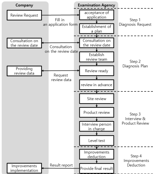
Fig. 4. Detail Procedure of Simplified Test Maturity Model for Examination Agency
