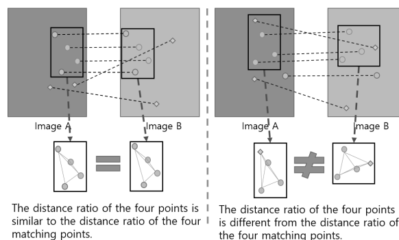
Fig. 15. How to Determine the Ratio of Distance Between Corresponding Points
