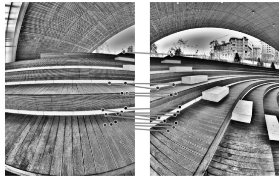
Fig. 4. Feature Matching
