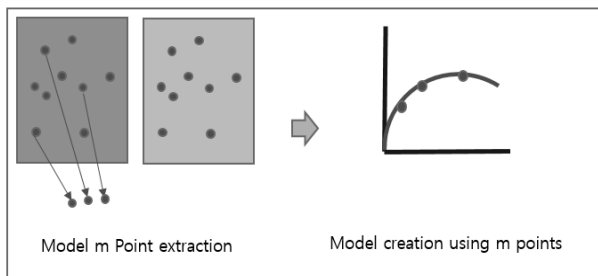
Fig. 5. Hypothesis Setting Step
