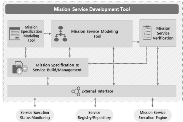
Fig. 5. Abstract Architecture of Mission Service Development Tool
