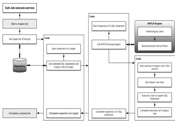
Fig. 6. Process of parsing process inspect rules
