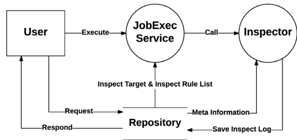
Fig. 2. Data Flow Diagram of SQL Auditor
