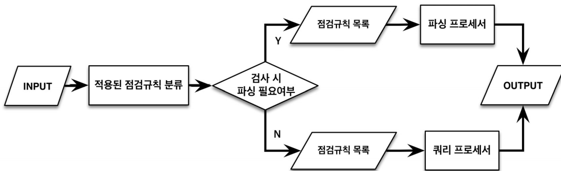
Fig. 3. Process of SQL Auditor
