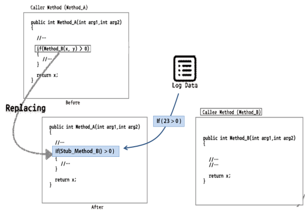
Fig. 4. Substitution Method of Calling Functions
