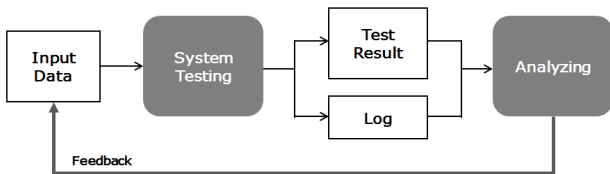
Fig. 1. Log-based Unit Testing Approach
