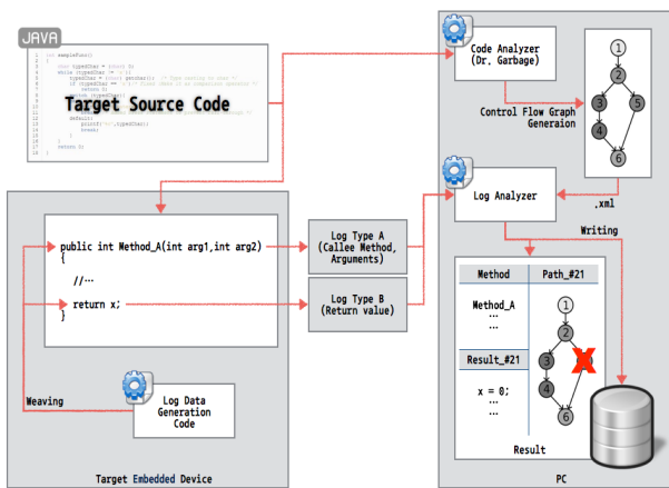
Fig. 2. Overview of Log-based Unit Testing Framework
