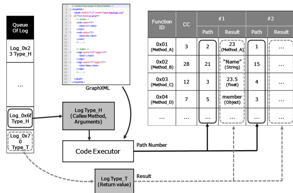
Fig. 3. Structure of Log Analyzer
