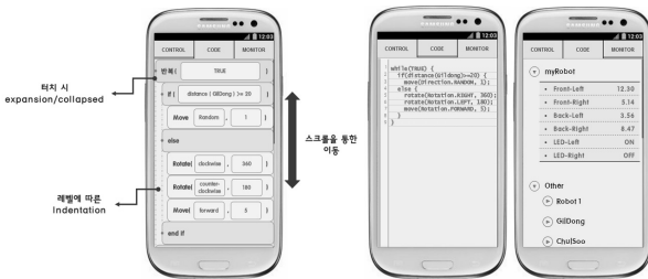
Fig. 2. Mobile Interface for Robot Programming
