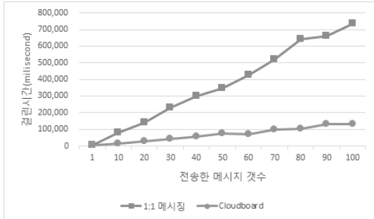
Fig. 6. Messaging Performance of Cloudboard
