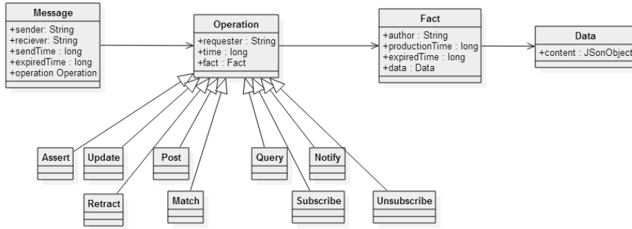
Fig. 5. Interface to the Cloudboard
