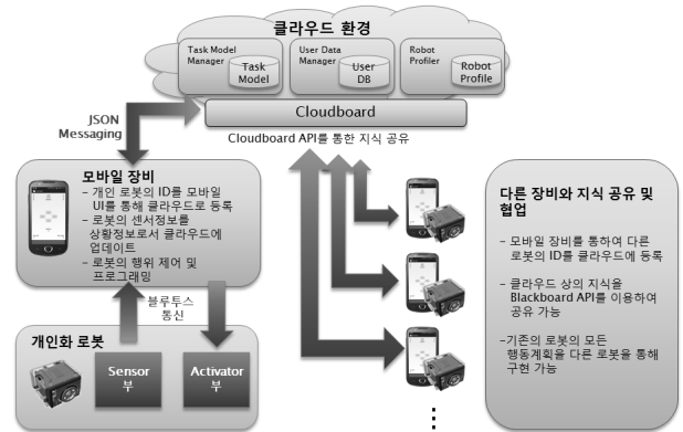
Fig. 4. Cloud Robot Programming Framework
