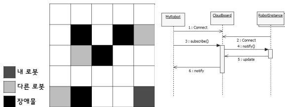
Fig. 3. Robot Programming in Cloud Environment
