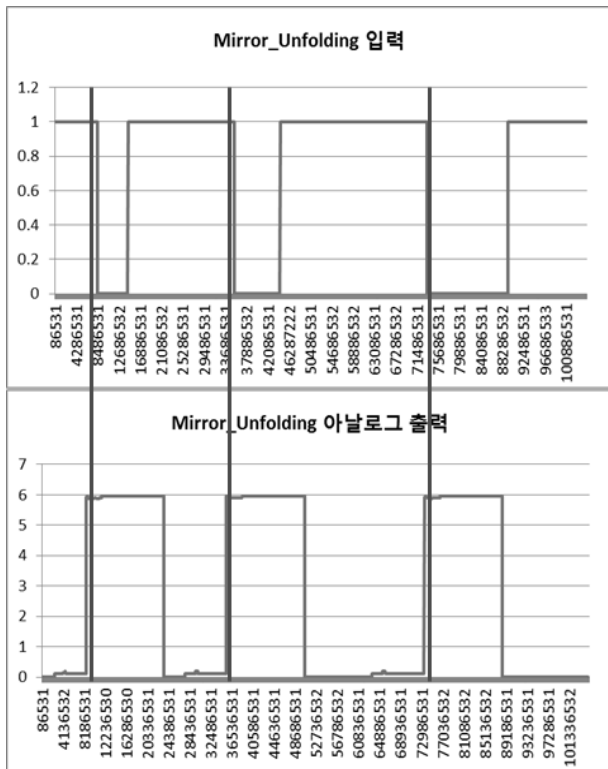
Fig. 7. For example, the driver's window control test result data
