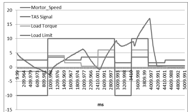
Fig. 6. For example, BLDC motor test results data
