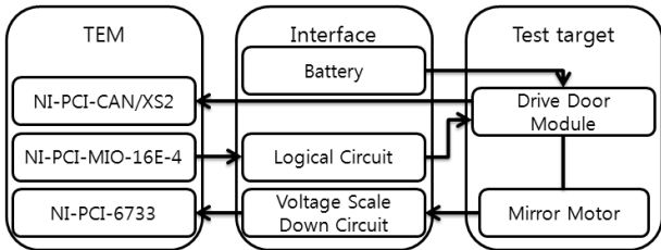
Fig. 4. Configuration of the driver's window control test
