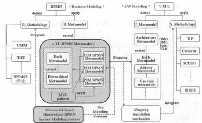
Fig. 1. Scope model of layered BPMN modeling approach
