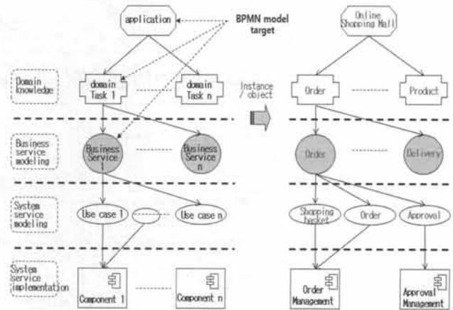
Fig. 3. Service construction of online shopping mall system
