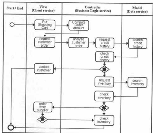
Fig. 11. MVC based Integrated service PIM BPMN model
