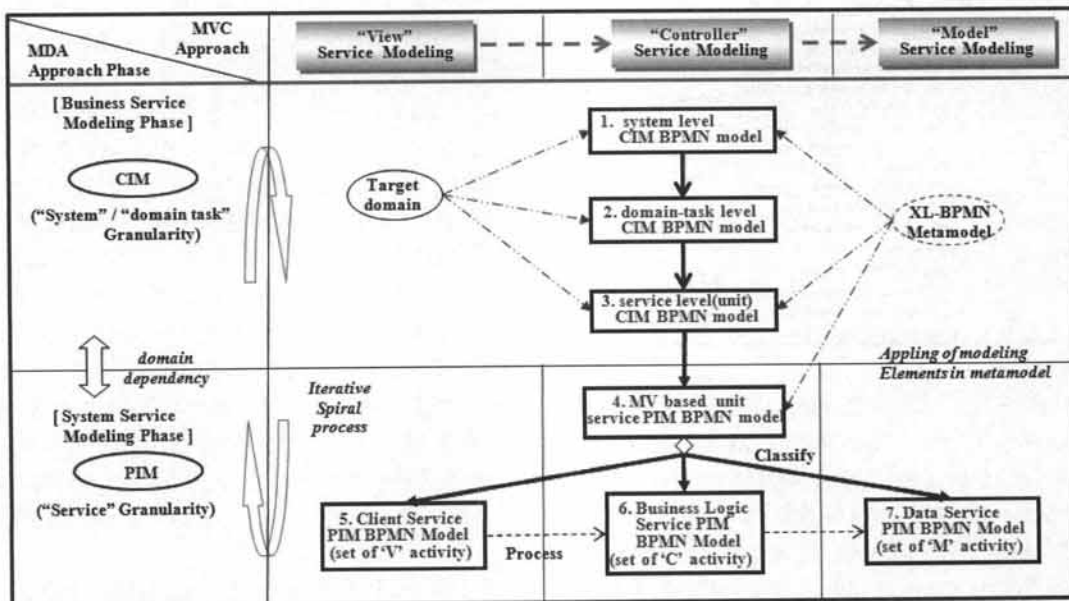
Fig. 7. Layered BPMN modeling architecture and process based on MDA/MVC
