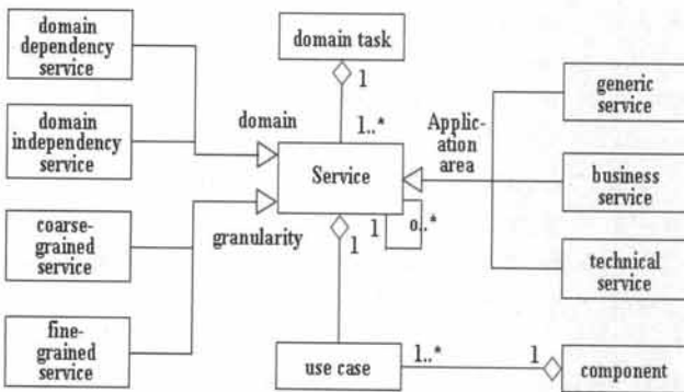
Fig. 2. Service metamodel
