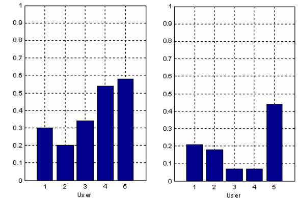
Fig. 14. Wrong recognition rate (L: Threshold value used, R: Fuzzy garbage model used)
