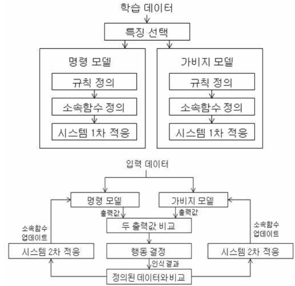
Fig. 18. Two stage user adaptation (Top: Offline-Batch, Bottom: Online-Incremental)
