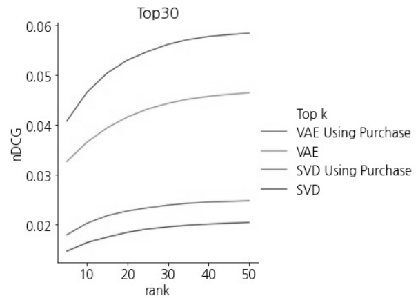
Fig. 5. Performance Evaluation using Top 30 Similar Customers
