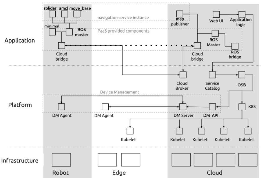
Fig. 3. ROS with Google Cloud
