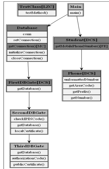
Fig. 5. Sample Code Before Refactoring
