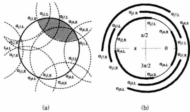
(Fig. 2) K-perimeter-coverage maintenance [7]. (a) segment of sensor s_i 's perimeter covered by s_{jn} ( n = \overline{1..8} ), and (b) the perimeter-coverage for the sensor s_i 's perimeter. For each sensor s_{jn} such that d(s_i, s_{jn}) \leq 2r , determine the angle of s_i 's arc, denoted by [\alpha_{jn,L}, \alpha_{jn,R}] , that is perimeter-covered by s_{jn} .
