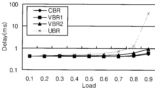
(c) 폴링 간격=0.2 ms
