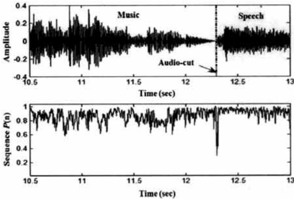
(Figure 5) Segmentation result using the proposed algorithm
