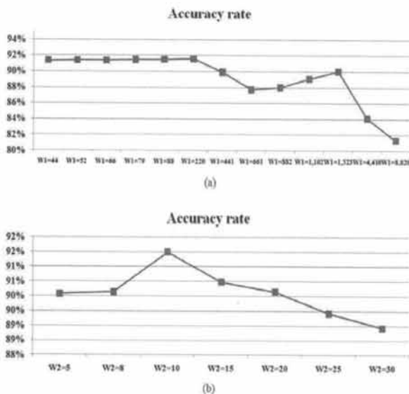
(Figure 3) Determining suitable window lengths with test data set. (a) window length W_1 to extract feature vectors, and (b) window length W_2 to compute parameter sequence P(n)
