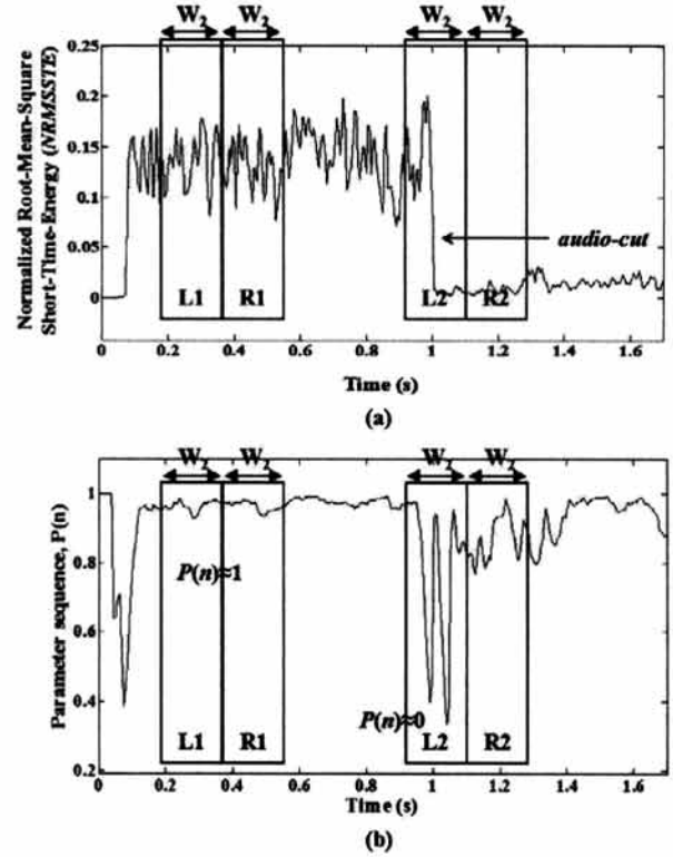
(Figure 2) Audio-cut versus non audio-cut. (a) RMS values in the processing windows, and (b) parameter sequence, P(n) , in the processing windows
