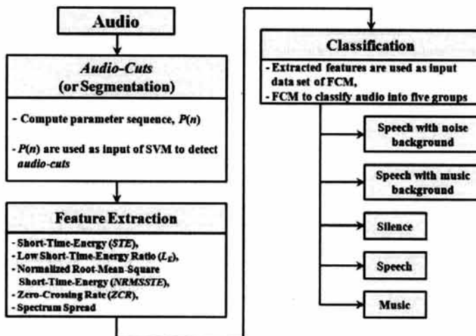
(Figure 1) Block diagram for the proposed audio segmentation and classification algorithm
