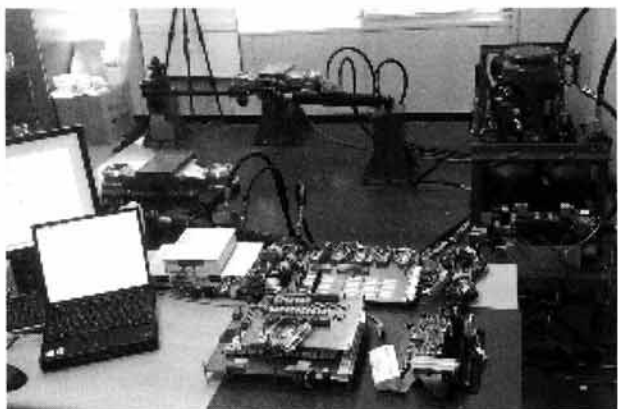
(그림 9) Hardware In the Loop System about AWS ECU
