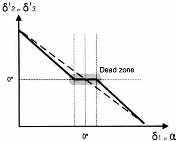
(그림 7) Determine desired rear angle from front angle
