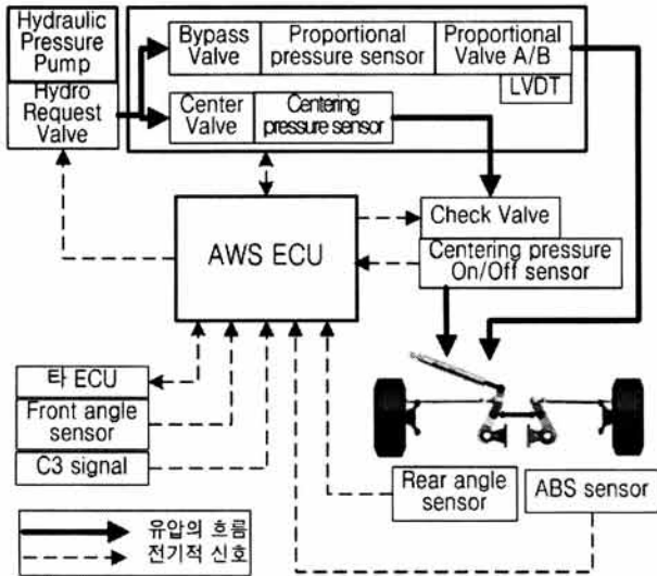
(그림 3) In-Out Structure of AWS System
