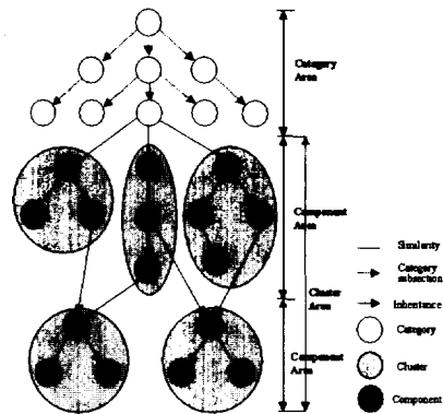
(그림 3) Embedded Three-tired Class Library Hierarchy
