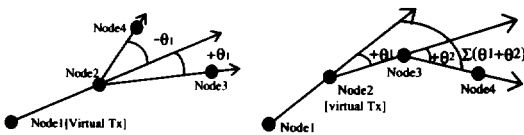
(Fig. 9) Decision of LOS/NLOS by the angles subtended between nodes
