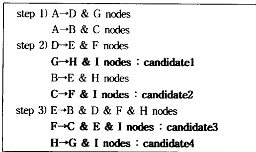
(Fig. 8) An instance process to find a path from A to I node
