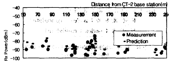
(Fig. 13) Comparison between measurement and prediction by building blockage
